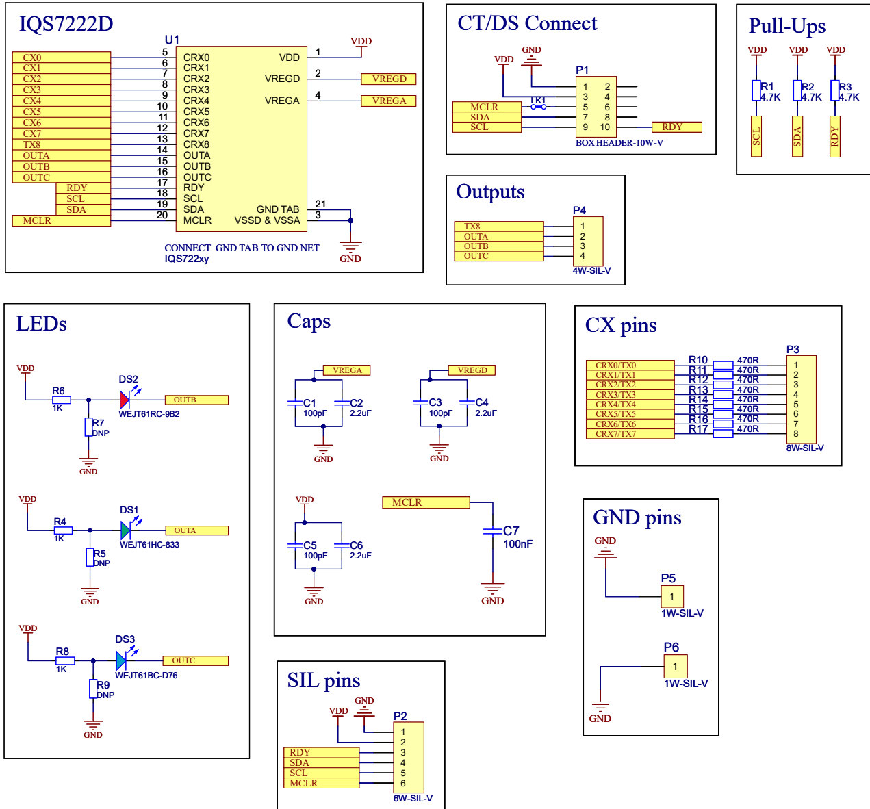
Figure 4.1: General-Purpose Stamp Reference Schematic
