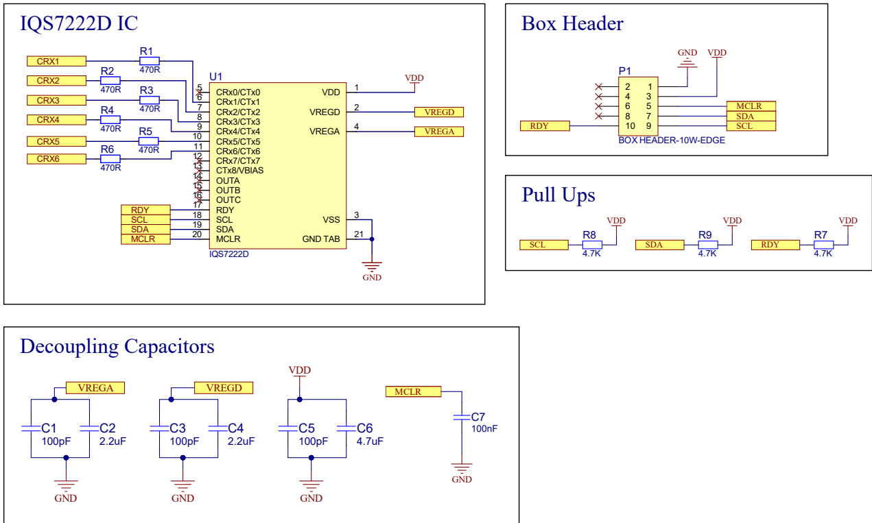
Figure 4.2: Trackpad Reference Schematic
