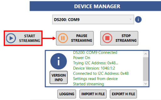
Figure 2.7: Message Dialogue Results from a Successful IQS7222D Connection
