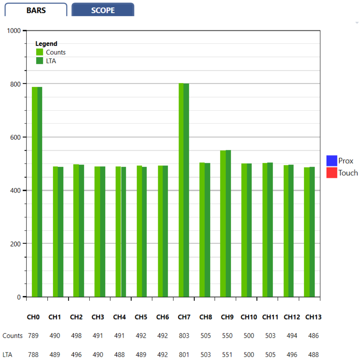
Figure 3.1: Streaming Graphs
