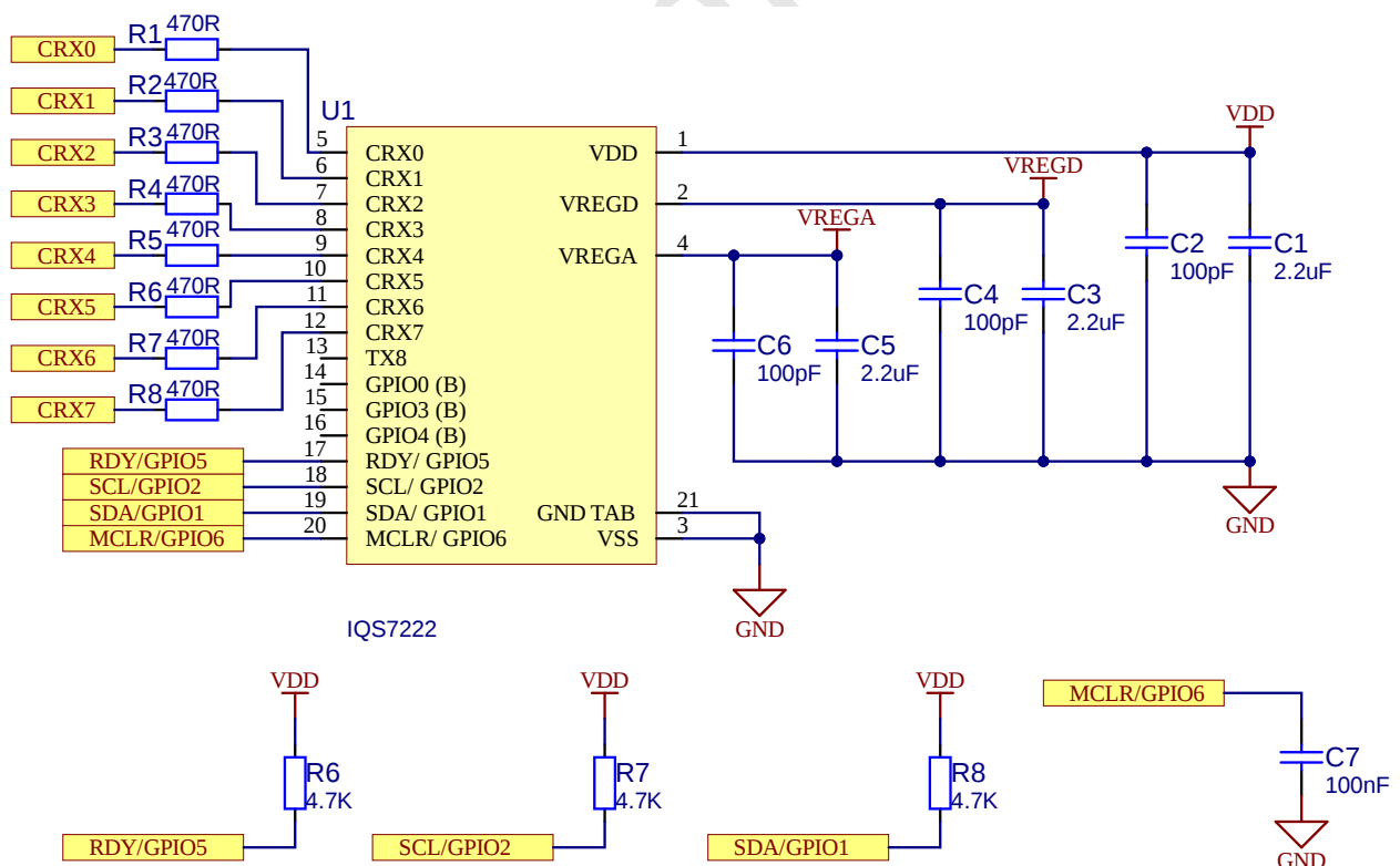
Figure 2.2: 8 Button Self Capacitance Reference Schematic
