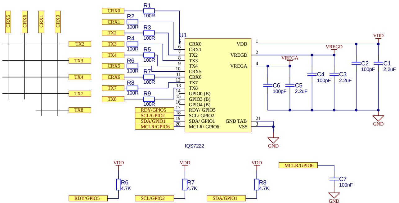
Figure 2.1: 18 Button Mutual Capacitance Reference Schematic
