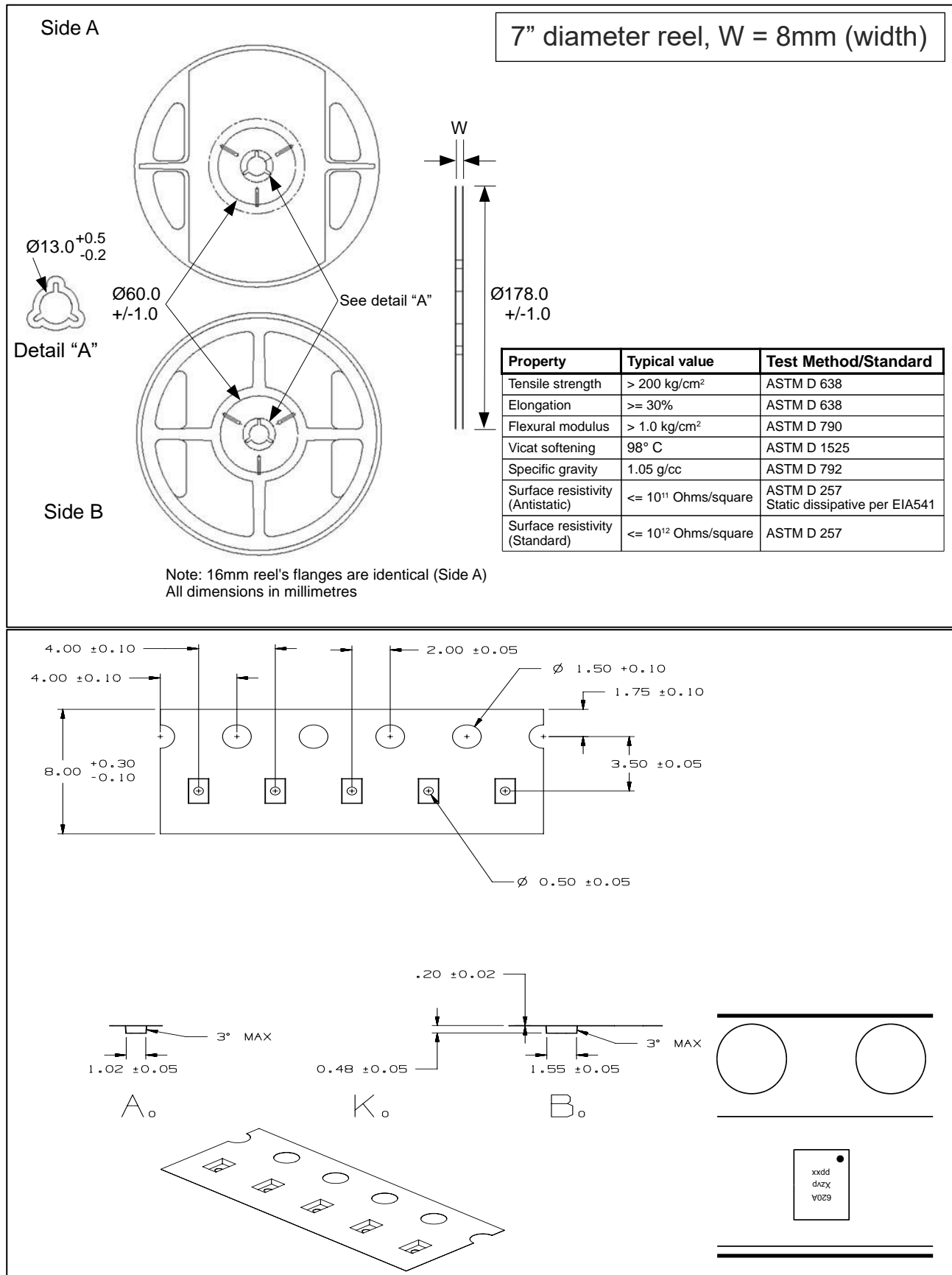
Figure 11.1 IQS620A WLCSP-9 tape & reel specification
