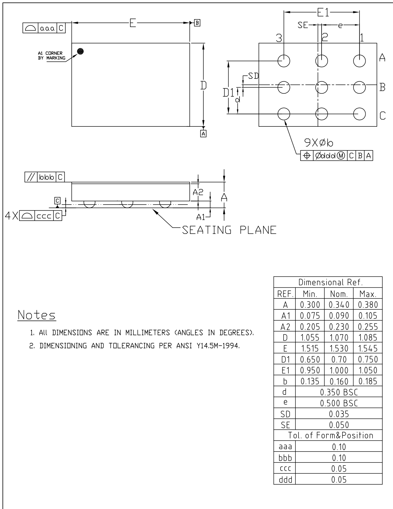
Figure 10.1 IQS620A WLCSP-9 package dimensions
