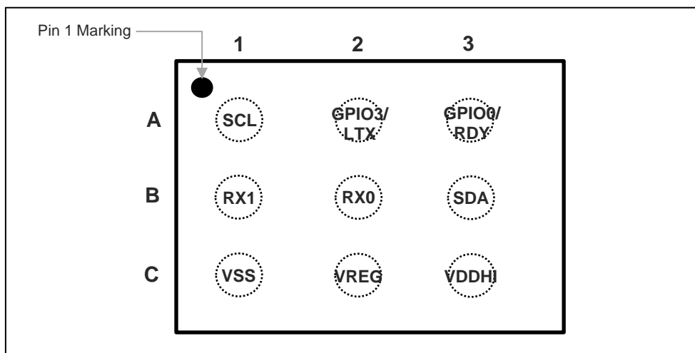
Figure 1.2 IQS620A pin-out (WLCSP-9 package top view; markings may differ)
