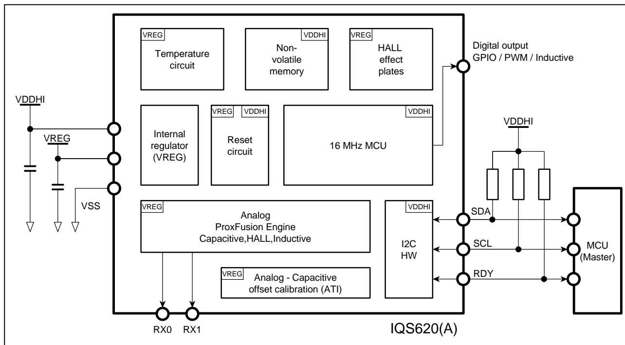
Figure 1.1 IQS620A functional block diagram
