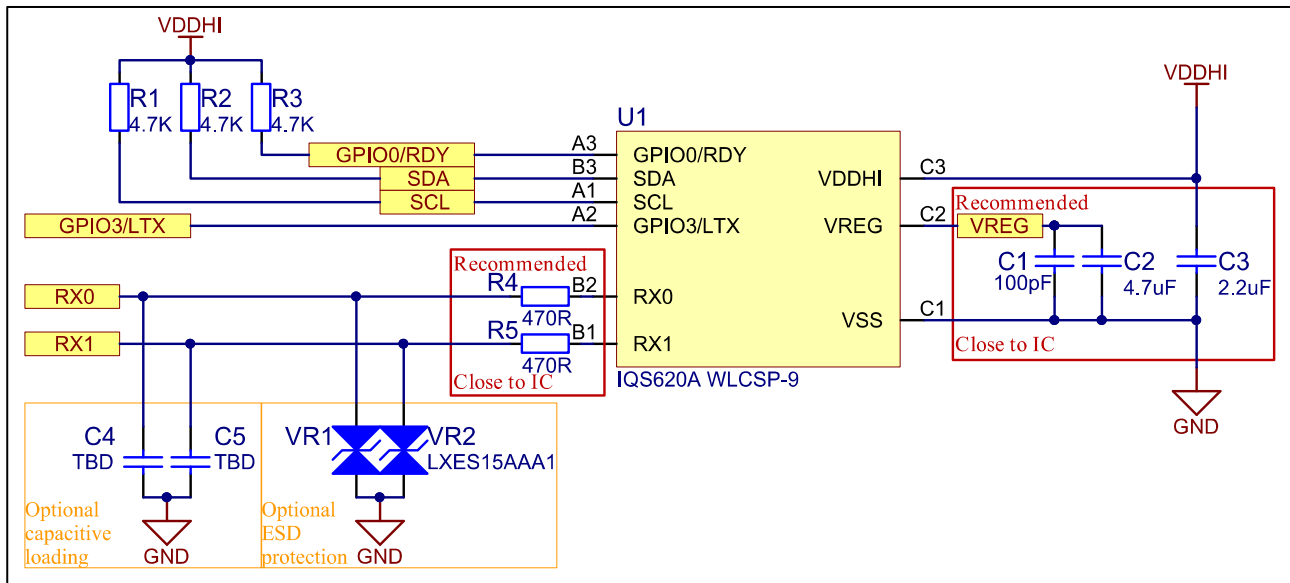
Figure 1.3 IQS620A WLCSP-9 reference schematic
