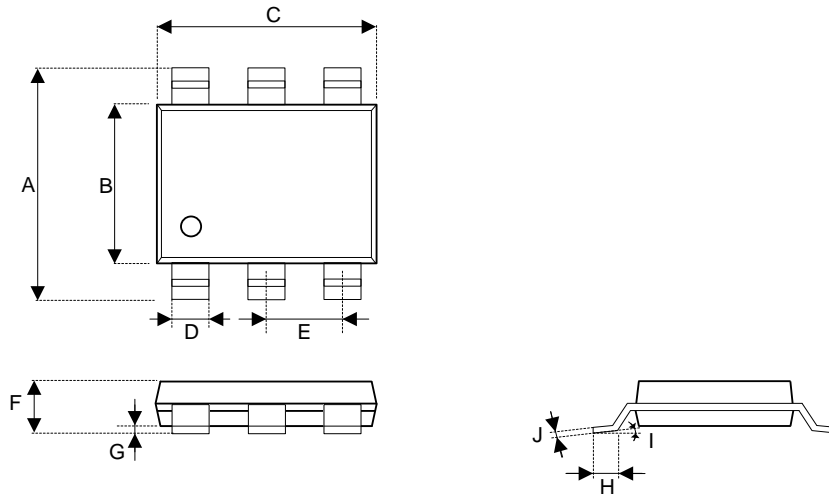
Figure 8.1 TSOT23-6 Packaging 4
