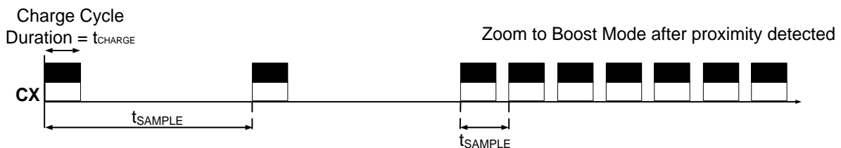
Figure 5.4: LP Modes: Charge cycles
