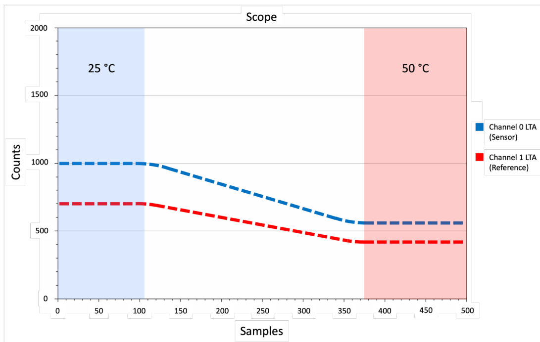
Figure 7.3: Example Scope View of a Device in a Temperature Characterisation Test
