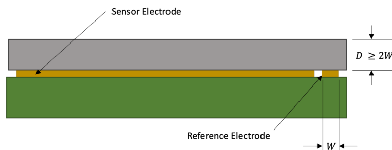
Figure 7.1: Illustration of the approximate width sizing of the reference electrode
