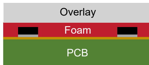
Figure 3.8: Foam filled in between overlay and electrode
