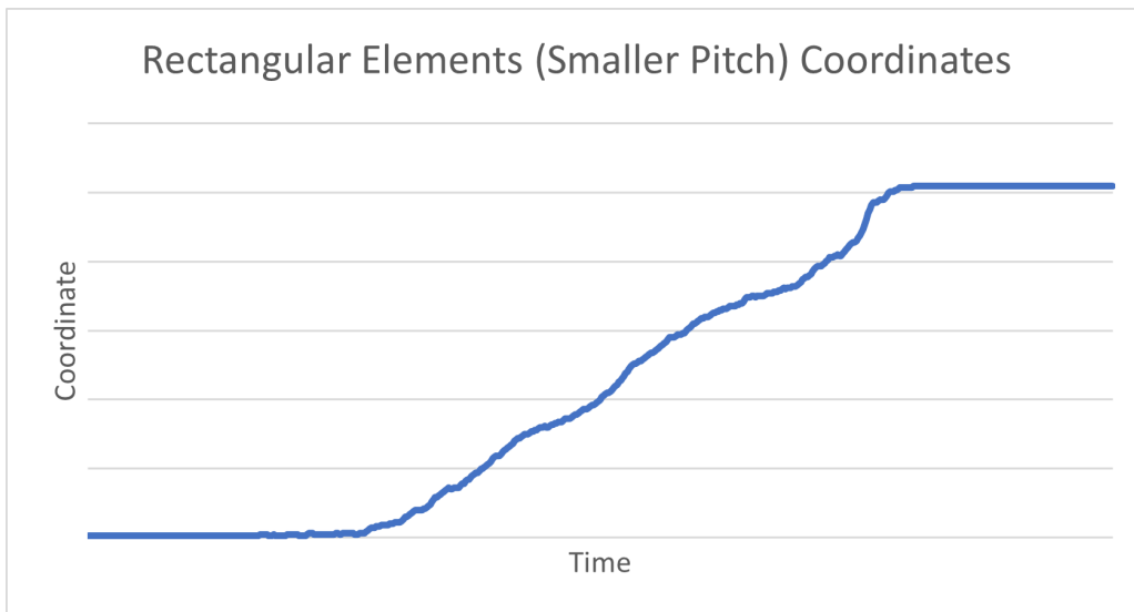
Figure 6.4: Self-capacitive slider with a smaller pitch
