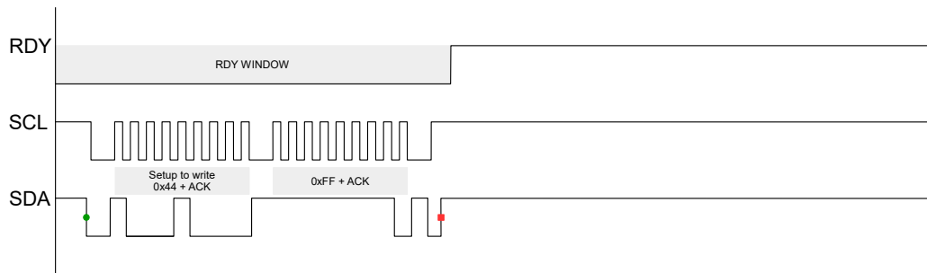
Figure 9.3: Force Stop Communication Sequence
