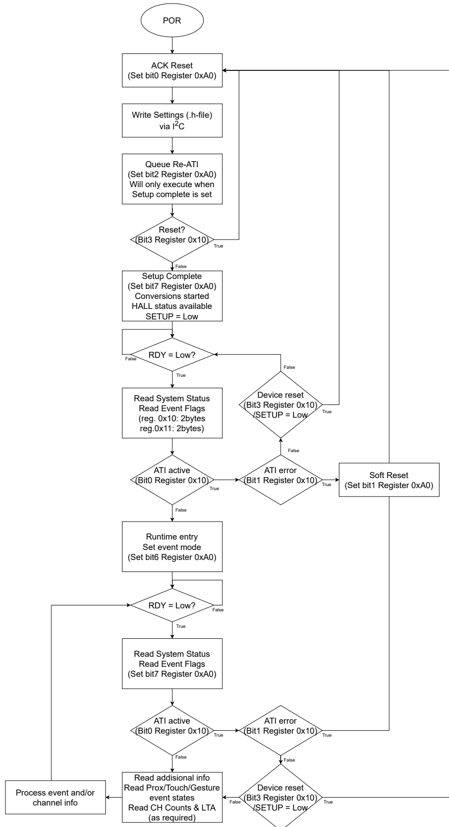
Figure 9.5: Program Flow Diagram
