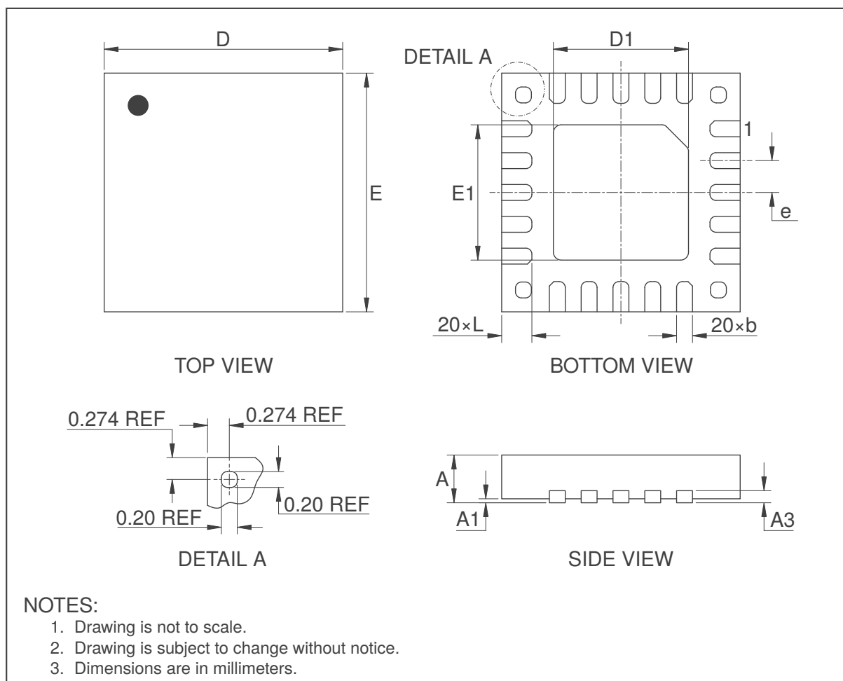
Figure 11.5: QFN (3x3)-20 (QNR) Package Outline Visual Description
