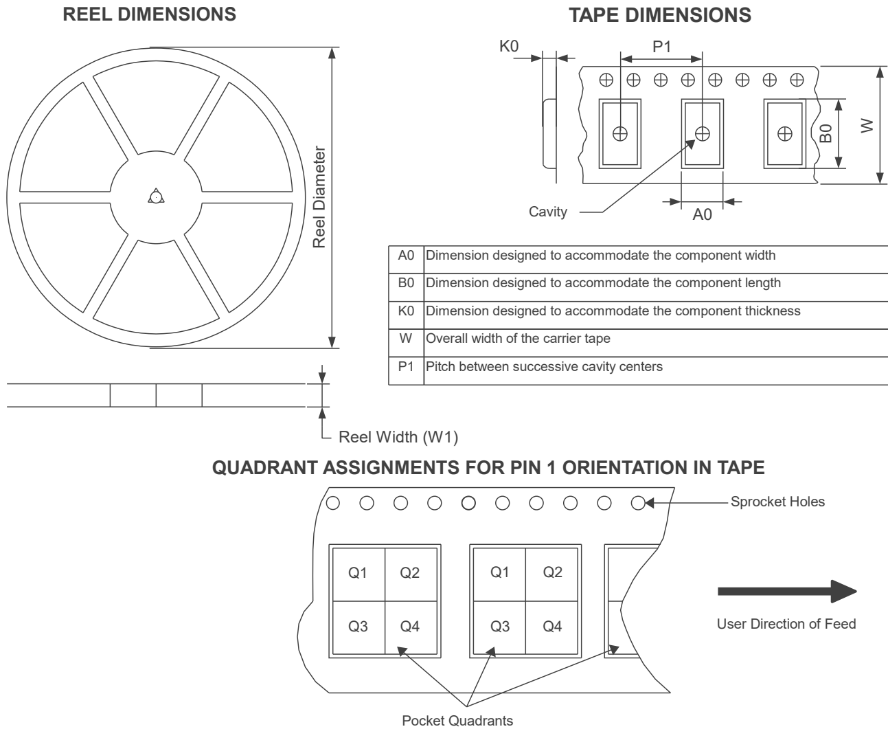
Figure 11.9: Tape and Reel Specification
