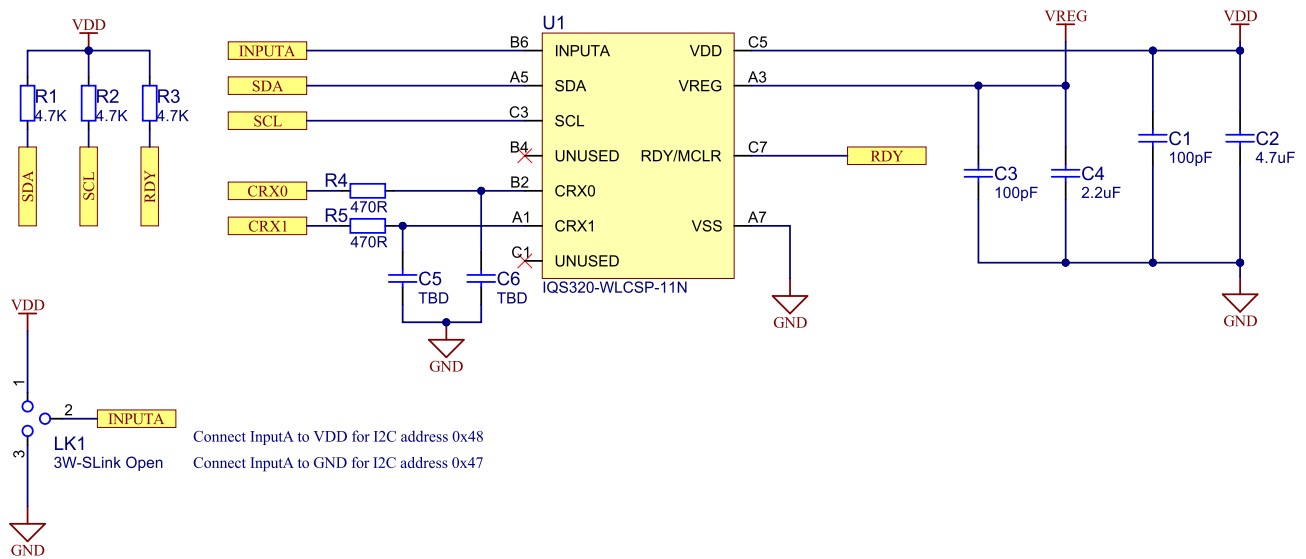
Figure 2.1: WLCSP11 I²C Reference Schematic
