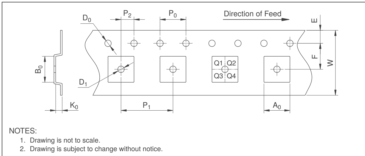
Figure 12.5: Carrier Tape Specification
