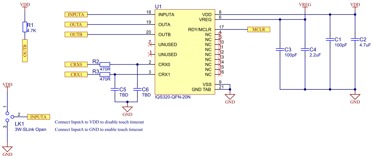
Figure 2.4: QFN20 Standalone Reference Schematic
