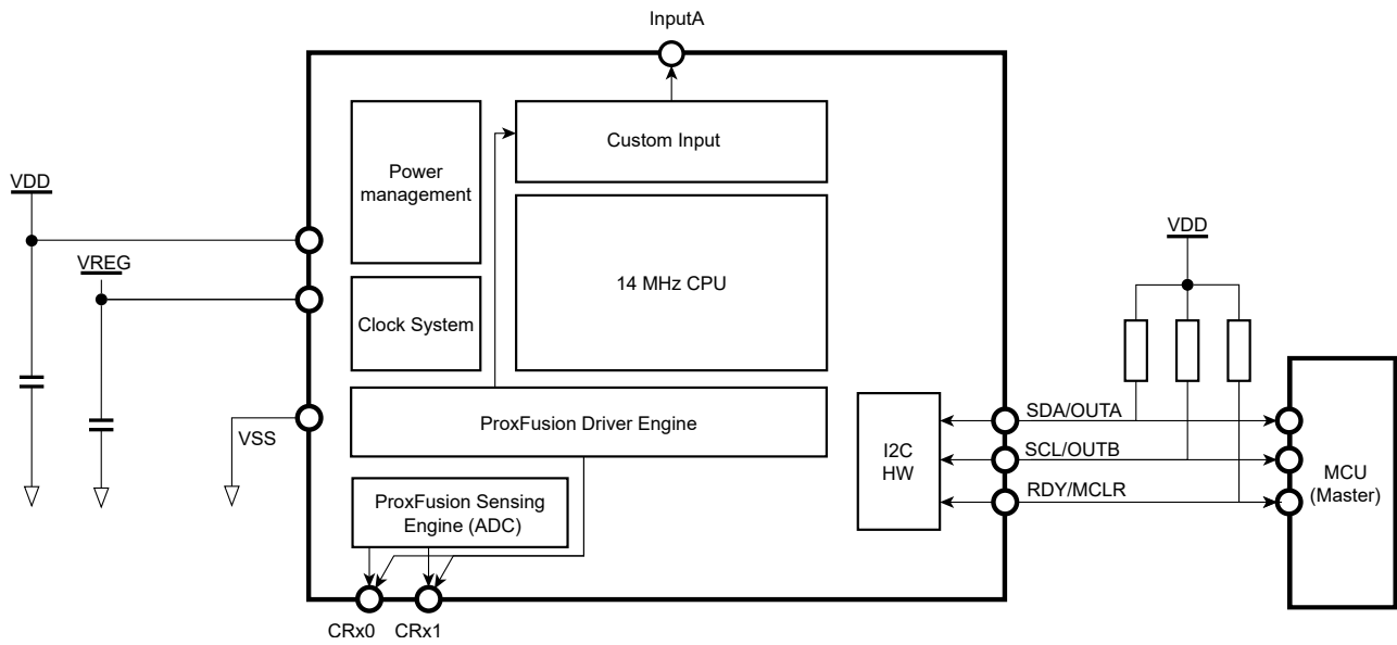
Figure 1.3: Functional Block Diagram
