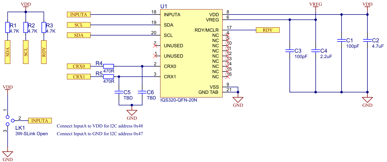
Figure 2.3: QFN20 I²C Reference Schematic
