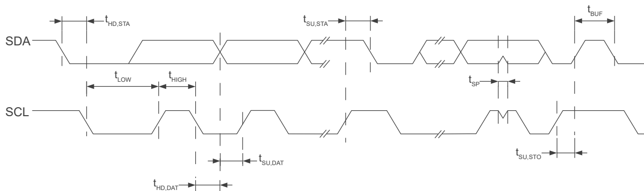
Figure 5.2: I 2 C Mode Timing Diagram
