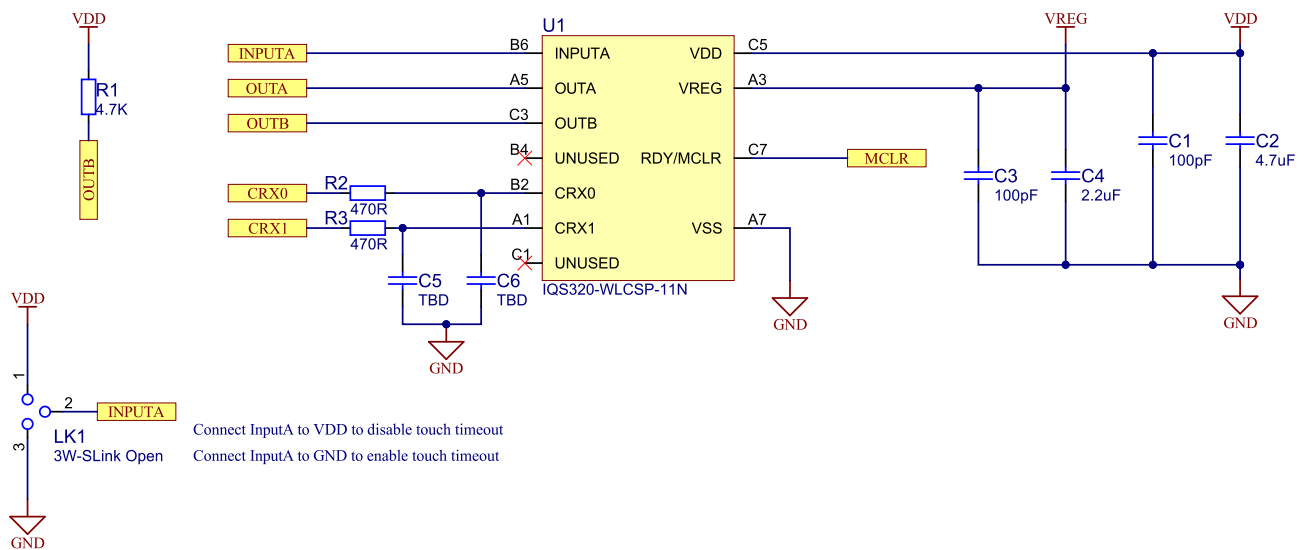
Figure 2.2: WLCSP11 Standalone Reference Schematic
