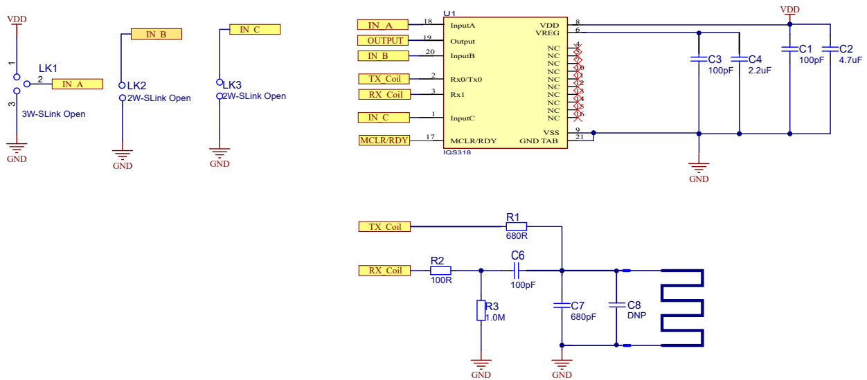
Figure 2.1: QFN20 Inductive Reference Schematic (IQS318-0xx, IQS318-1xx, and IQS318-2xx) i
