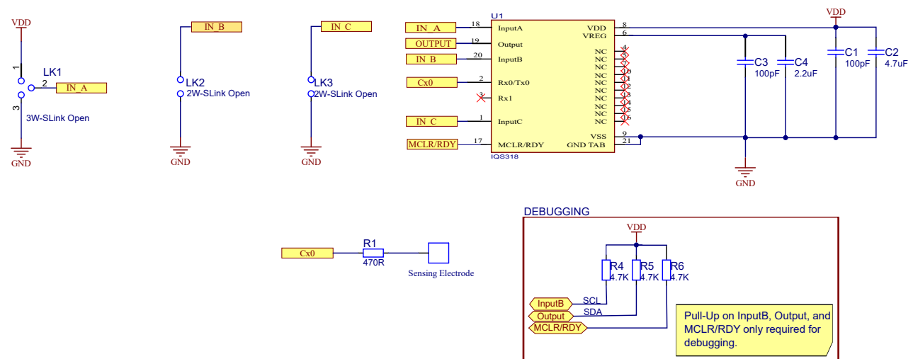
Figure 2.2: QFN20 Self-Capacitive Reference Schematic (IQS318-5xx) i
