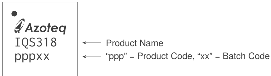
Figure 9.2: IQS318-QFN20 Package Top Marking
