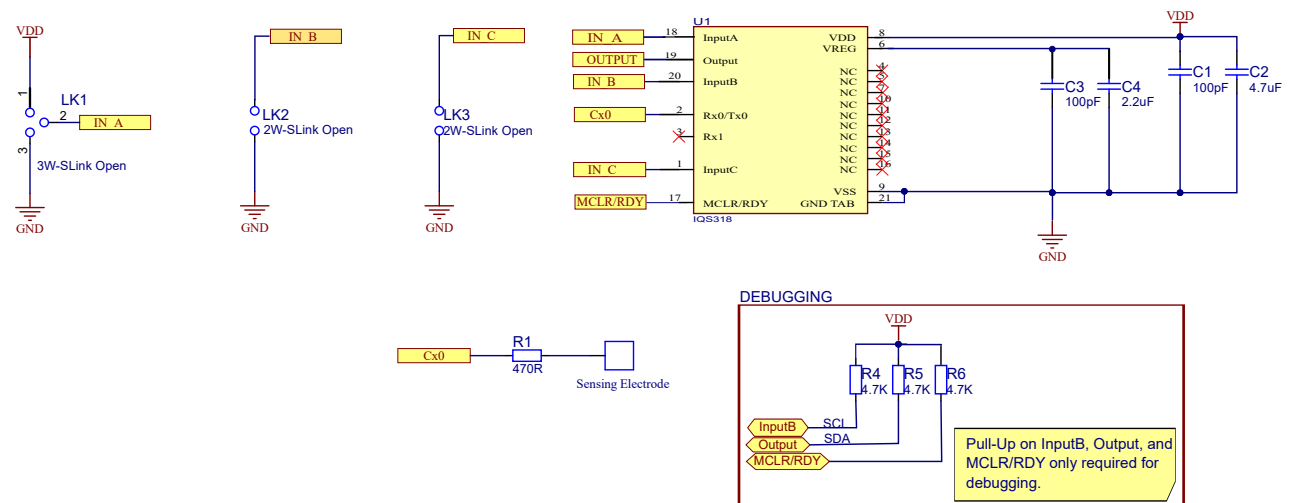
Figure 2.4: QFN20 Self-Capacitive Reference Schematic (IQS318-5xx) i
