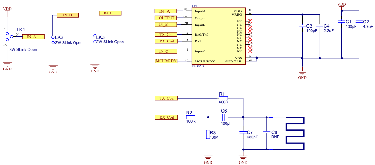
Figure 2.3: QFN20 Inductive Reference Schematic (IQS318-0xx, IQS318-1xx, and IQS318-2xx) i
