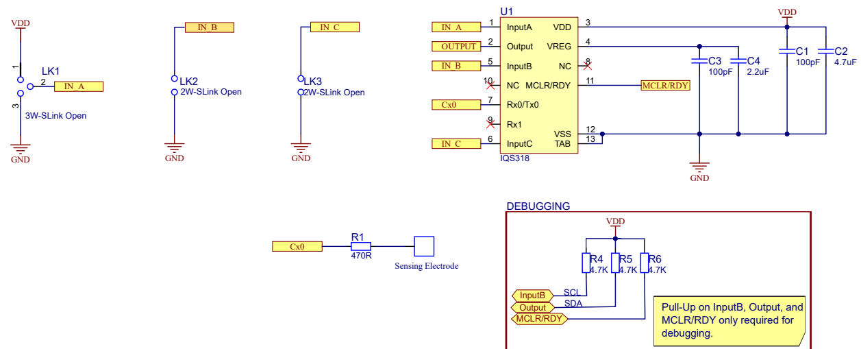
Figure 2.2: DFN12 Self-Capacitive Reference Schematic (IQS318-5xx) i
