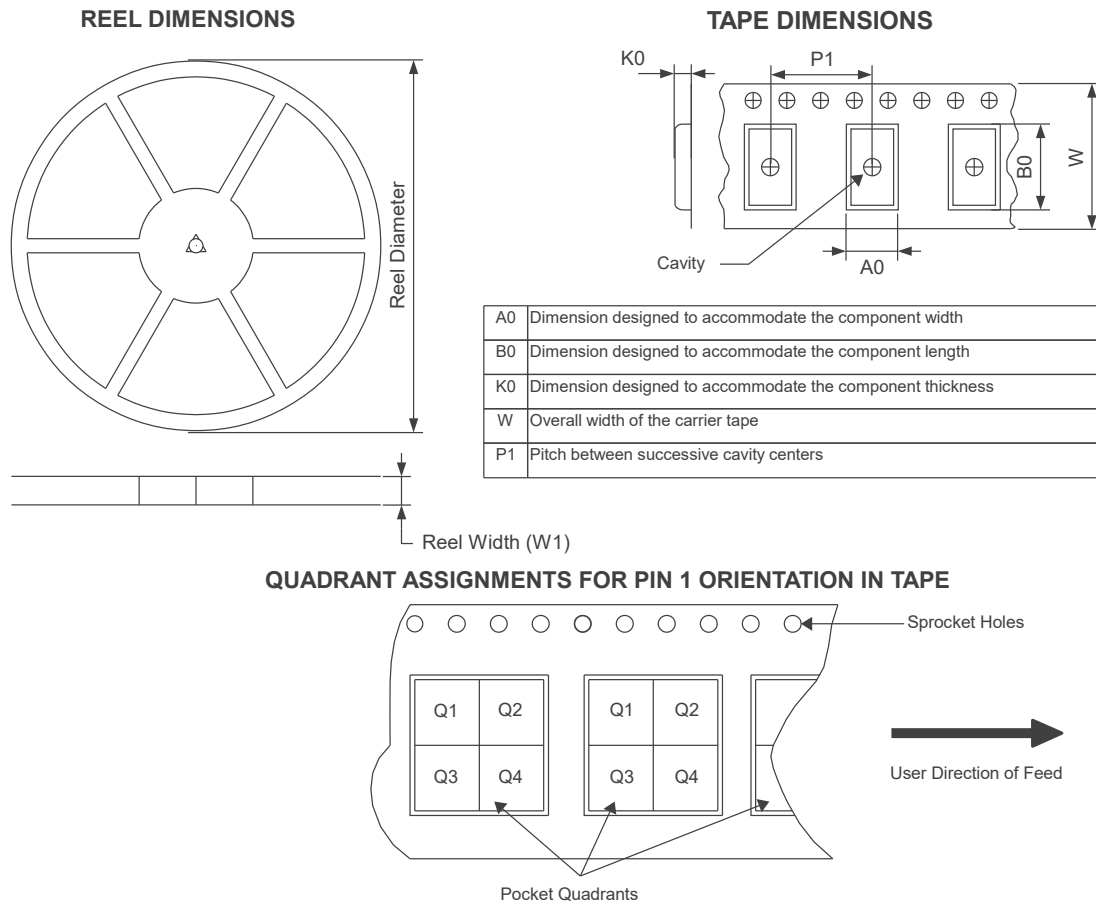
Figure 13.1: Tape and Reel Specification
