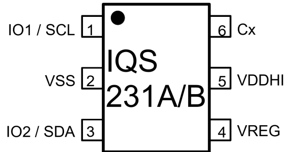
Figure 2.1: IQS231A/B TSOT23-6 Pin-out
