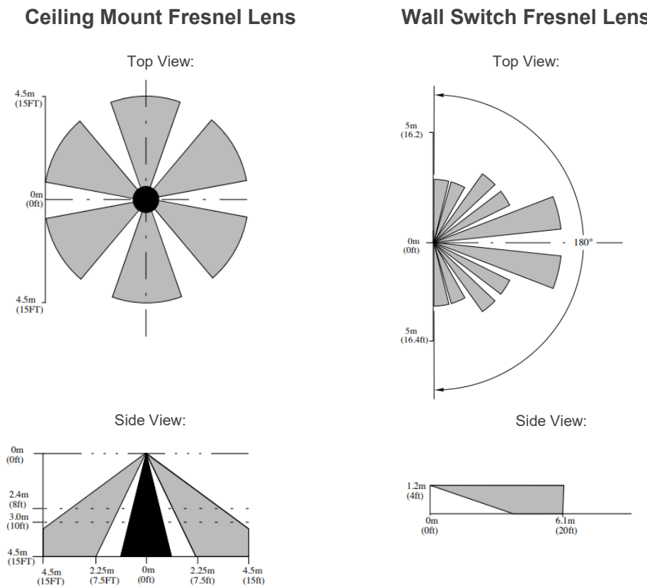
Figure 5-2: Different Fresnel Lenses (Adapted from: www.fresneltech.com )
