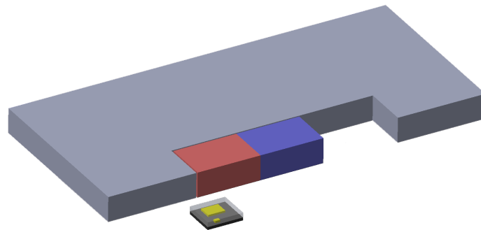
Figure 8-2: Hall-sensor slide switch
