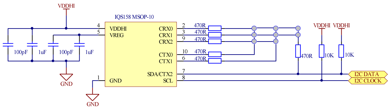
Figure 4.1 Reference Design.
