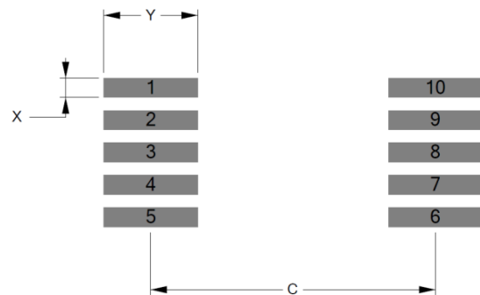
Figure 12.4 MSOP-10 Footprint.
