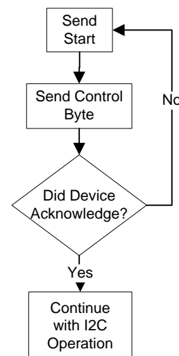
Figure 9.2 ACK Polling.
