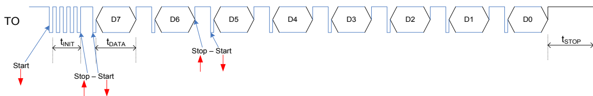
Figure 9.1 Serial data streaming: 1-wire streaming (Debug Mode)
