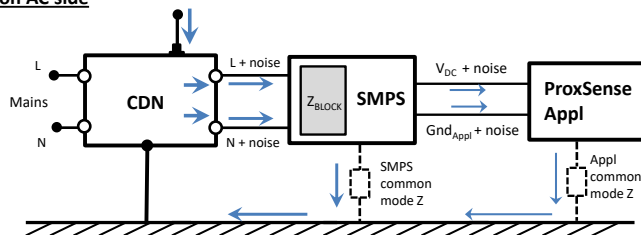
Figure 1: Injecting common mode noise into a DUT with two AC power lines, using a CDN.
